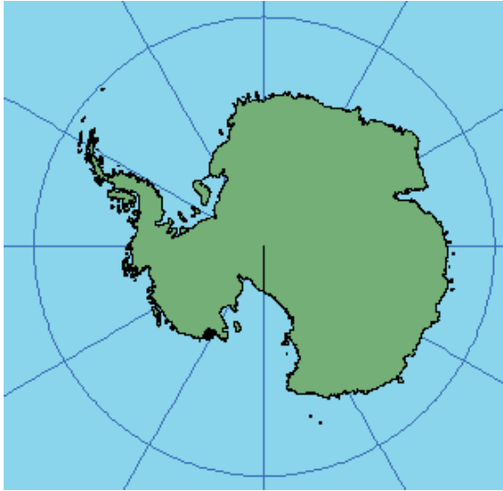
Central meridian is 0°, and latitude of origin is 90° S.
