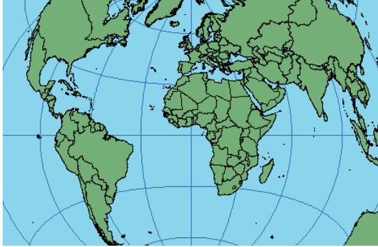
The center of the projection is 0°, 0°.
